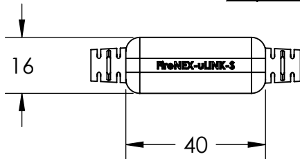
Repeater Unit
